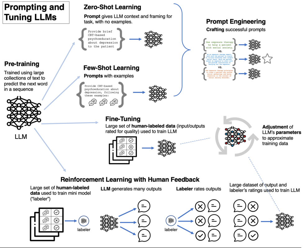
Fig. 1 | Methods for tailoring clinical large language models. Figure was designed using image components from Flaticon.com.
